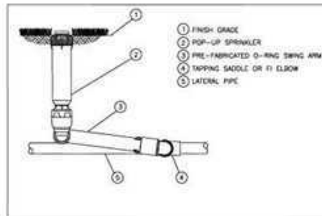
ROTOR POP-UP SPRINKLER 8005
