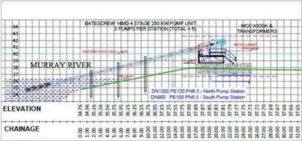
PROFILE - PUMPS (SCALE 1:100)
