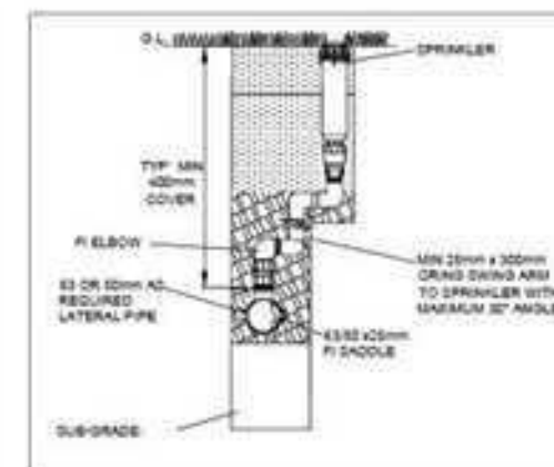
TYPICAL LATERAL TRENCH/SPRINKLER SECTION
