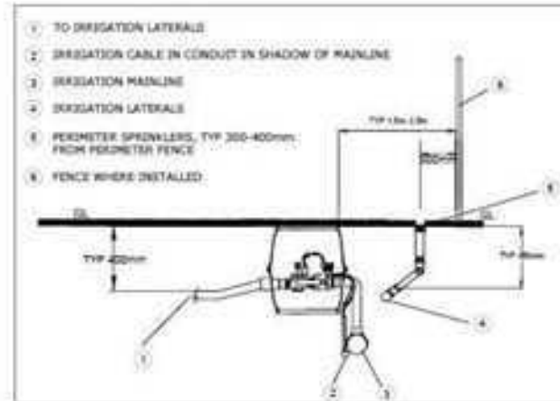
TYPICAL CROSS SECTION OF IRRIGATION
